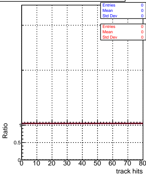
— DQM_correctCheck3_mu_pt0p1to1_eta2p0to2p5
