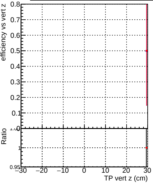
Efficiency vs TP vert z (cm) Legend: DQM_correctCheck2_mu_pt1to1000_eta2p5to4p0 DQM_original_mu_pt1to1000_eta2p5to4p0
