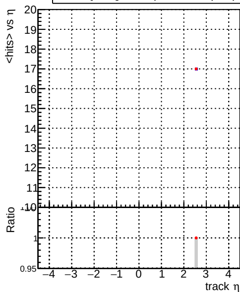
mean hits vs \eta DQM_correctCheck2_mu_pt1to1000_eta2p5to4p0 DQM_original_mu_pt1to1000_eta2p5to4p0
