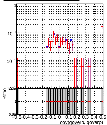
DQM_correctCheck2_mu_pt1to1000_eta2p5to4p0 DQM_original_mu_pt1to1000_eta2p5to4p0
