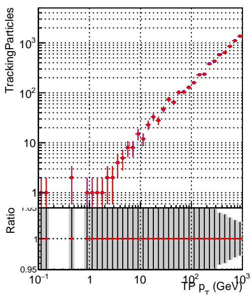
Legend: DQM_correctCheck2_mu_pt1to1000_eta2p5to4p0 (blue line with error bars), DQM_original_mu_pt1to1000_eta2p5to4p0 (red line with error bars)
