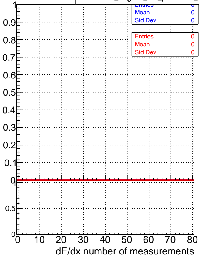
■ DQM_correctCheck2_mu_pt1to1000_eta2p5to4p0 ● DQM_original_mu_pt1to1000_eta2p5to4p0
