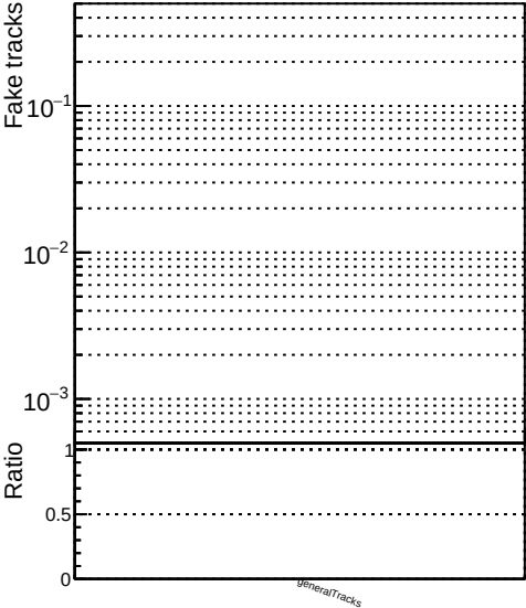
Number of fake tracks vs collection Legend: DQM_correctCheck2_mu_pt1to1000_eta2p0to2p5 DQM_original_mu_pt1to1000_eta2p0to2p5
