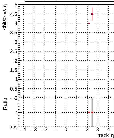
— DQM_correctCheck2_mu_pt1to1000_eta2p0to2p5 — DQM_original_mu_pt1to1000_eta2p0to2p5
