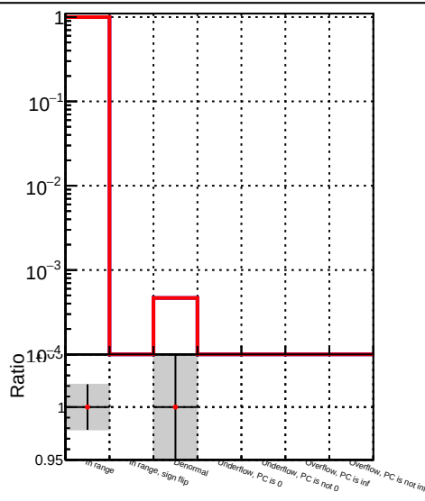
DQM_correctCheck2_mu_pt1to1000_eta2p0to2p5 DQM_original_mu_pt1to1000_eta2p0to2p5
