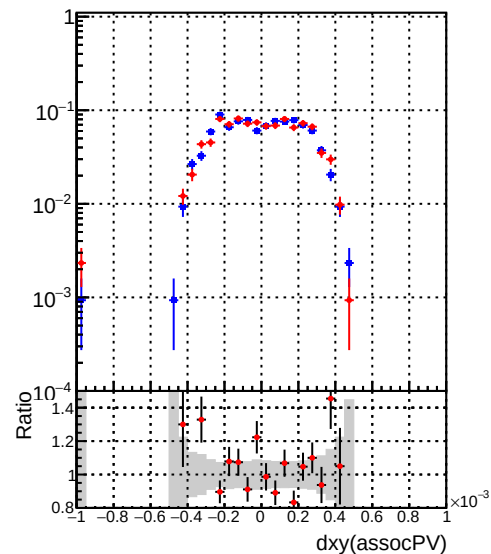
DQM_correctCheck2_mu_pt1to1000_eta2p0to2p5 DQM_original_mu_pt1to1000_eta2p0to2p5
