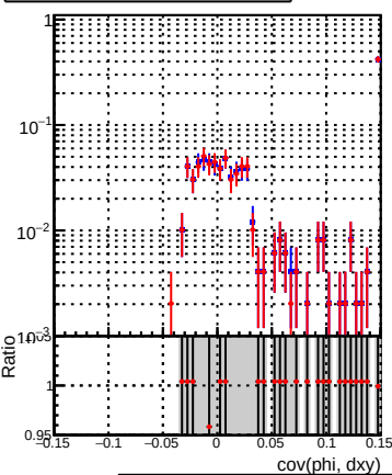
(PacketCandidate::bestTrack() - reco::Track)reco::Track in cov(phi, dxy)
