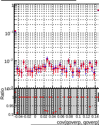
DQM_correctCheck2_mu_pt1to1000_eta2p0to2p5 DQM_original_mu_pt1to1000_eta2p0to2p5
