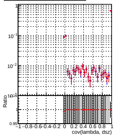
(PackedCandidate::bestTrack() - reco::Track)(reco::Track in cov(lambda, dsz) and underflow and overflow)
