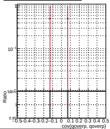
DQM_correctCheck2_mu_pt1to1000_eta2p0to2p5 DQM_original_mu_pt1to1000_eta2p0to2p5
