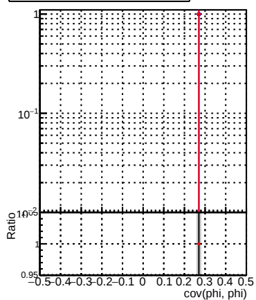
(PackedCandidate::bestTrack() - reco::Track)(reco::Track in cov(phi, phi) and underflow and overflow)
