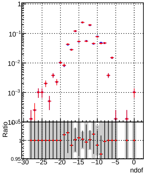
PackedCandidate Legend: DQM_correctCheck2_mu_pt1to1000_eta2p0to2p5 DQM_original_mu_pt1to1000_eta2p0to2p5
