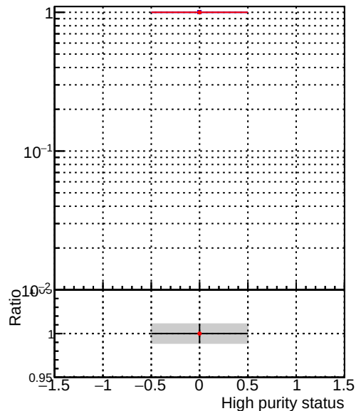
PackedCandidate Legend: DQM_correctCheck2_mu_pt1to1000_eta2p0to2p5 DQM_original_mu_pt1to1000_eta2p0to2p5
