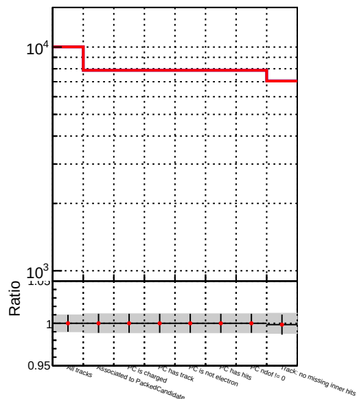
PackedCandidate Legend: DQM_correctCheck2_mu_pt1to1000_eta2p0to2p5 DQM_original_mu_pt1to1000_eta2p0to2p5
