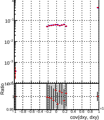
(PacketCandidate::bestTrack() - reco::Track)reco::Track in cov(dxy, dxy)
