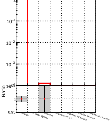
(PacketCandidate::bestTrack() - reco::Track)reco::Track in cov(dxy, dxy) status
