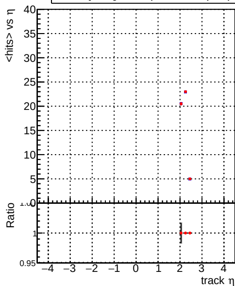
mean hits vs \eta Legend: DQM_correctCheck2_mu_pt1to1000_eta2p0to2p5 (blue line with dots), DQM_original_mu_pt1to1000_eta2p0to2p5 (red line with dots)
