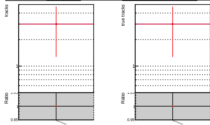
N of reco track vs. \chi^2 —•— DQM_correctCheck2_mu_pt1to1000_eta2p0to2p5 —•— DQM_original_mu_pt1to1000_eta2p0to2p5
