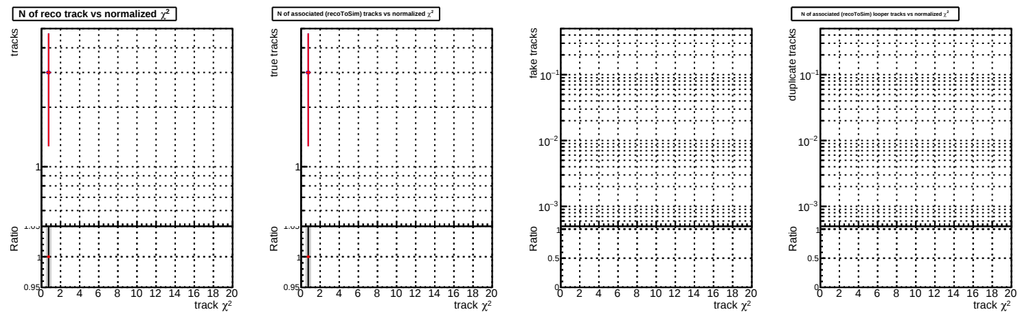
N of reco track vs. \chi^2 —•— DQM_correctCheck2_mu_pt1to1000_eta2p0to2p5 —•— DQM_original_mu_pt1to1000_eta2p0to2p5
