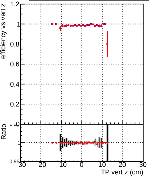
Efficiency vs vert z Legend: DQM_correctCheck2_mu_pt1to1000_eta2p0to2p5 (blue line with dots) DQM_original_mu_pt1to1000_eta2p0to2p5 (red line with dots)
