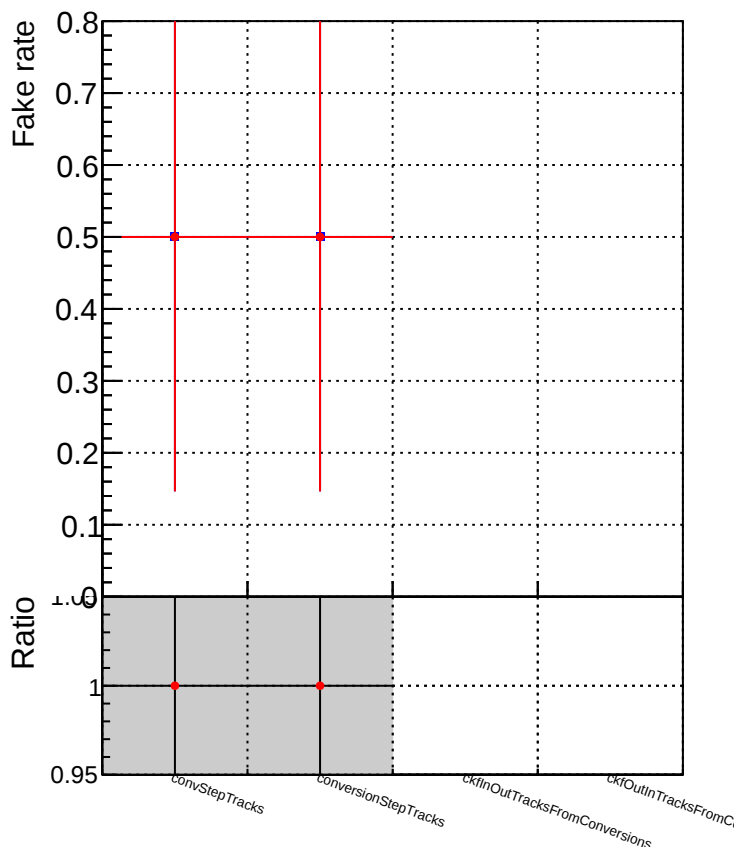
Fakerate vs collection
