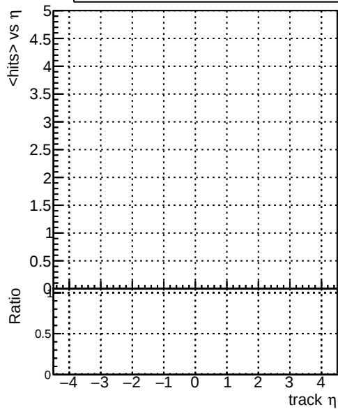
mean hits — DQM_correctCheck2_mu_pt1to1000_eta2p0to2p5 — DQM_original_mu_pt1to1000_eta2p0to2p5
