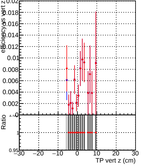
Efficiency vs. TP vert z (cm) vs. Sim. PV z (cm) Legend: DQM_correctCheck2_mu_pt1to1000_eta2p0to2p5 (blue line) DQM_original_mu_pt1to1000_eta2p0to2p5 (red line)
