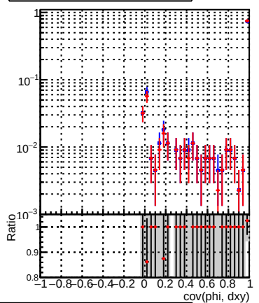
(PacketCandidate::bestTrack() - reco::Track)reco::Track in cov(phi, dxy) status with over- and underflow, and sign flip
