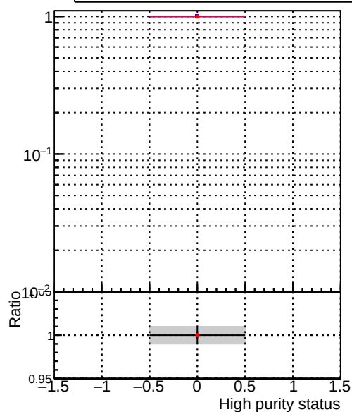
DQM_original_mu_pt1to1000_eta1p5to2p0
