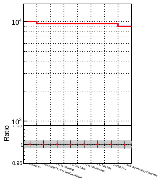
DQM_correctCheck2_mu_pt1to1000_eta1p5to2p0
