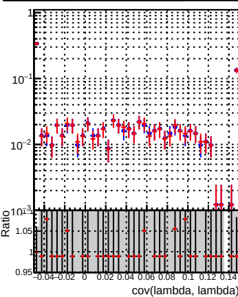
— DQM_correctCheck2_mu_pt1to1000_eta1p5to2p0 — DQM_original_mu_pt1to1000_eta1p5to2p0
