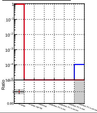
— DQM_correctCheck2_mu_pt1to1000_eta1p5to2p0 — DQM_original_mu_pt1to1000_eta1p5to2p0
