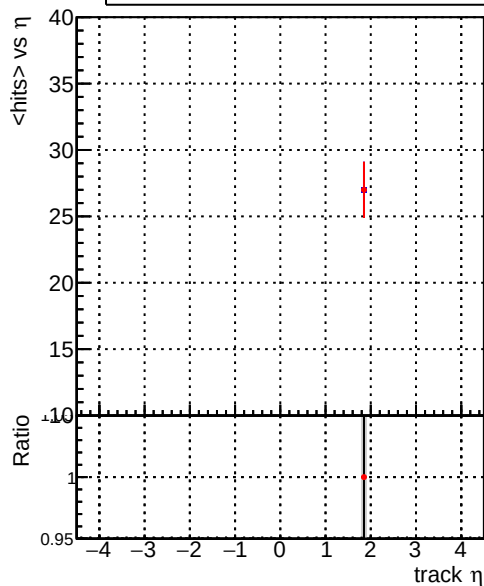
DQM_original_mu_pt1to1000_eta1p5to2p0
