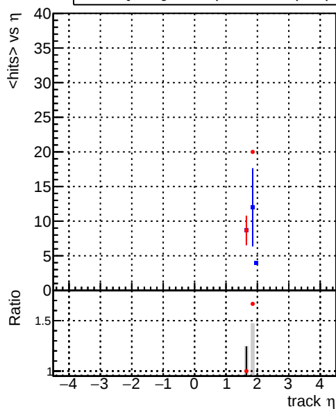
— DQM_correctCheck2_mu_pt1to1000_eta1p5to2p0 — DQM_original_mu_pt1to1000_eta1p5to2p0
