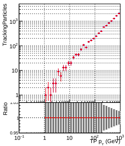
Legend: DQM_correctCheck2_mu_pt1to1000_eta1p5to2p0 (blue line), DQM_original_mu_pt1to1000_eta1p5to2p0 (red line)
