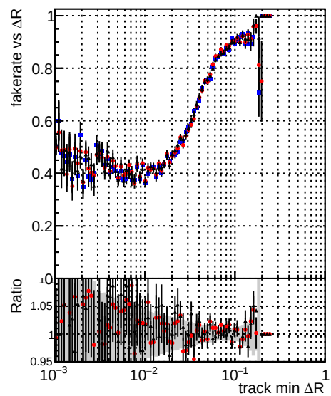
—•— DQM_mkFit_TToriginal —•— DQM_mkFit_TT_JanUpdate-noErr —•— DQM_mkFit_TT_JanUpdate-noErr1H
