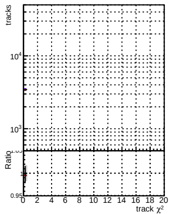
N of reco track vs. \chi^2 for different fit types
