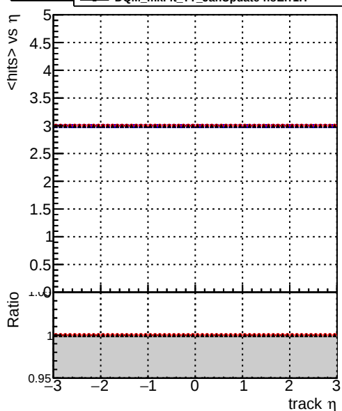
mean hits vs \eta DQM_mkFit_TToriginal DQM_mkFit_TT_JanUpdate-noErr DQM_mkFit_TT_JanUpdate-noErr1H
