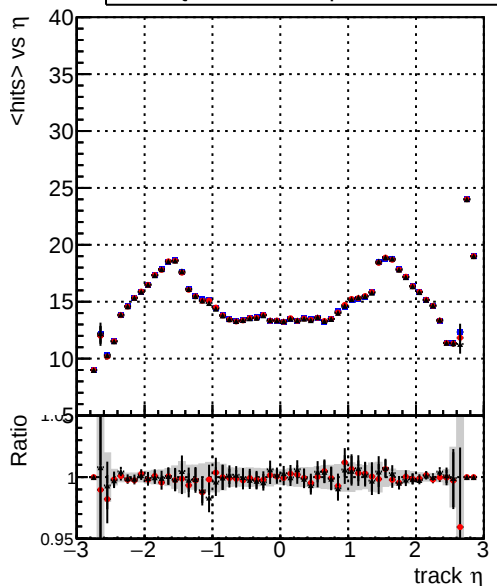
mean hits DQM_mkFit_TToriginal DQM_mkFit_TT_JanUpdate-noErr DQM_mkFit_TT_JanUpdate-noErr1H
