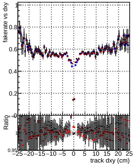
Fake rate vs d DOM mkFit TToriginal DOM mkFit TT JanUpdate-noErr DOM mkFit TT JanUpdate-noErr1H
