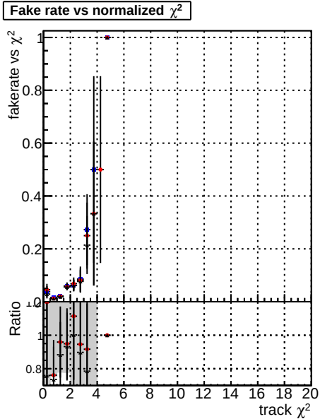
Fake rate vs. \chi^2 Legend: DOM mkFit T (blue), JanUpdate-noErr (red), JanUpdate-noErr1H (black)
