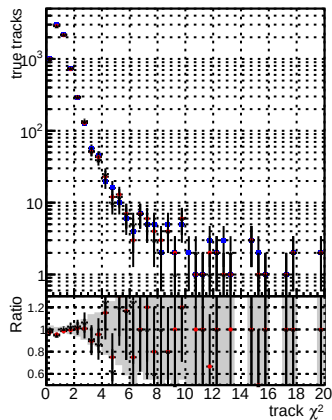
True tracks vs. \chi^2
