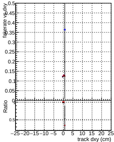
DOM mkFit TToOriginal DOM mkFit JanUpdate-noErr1H
