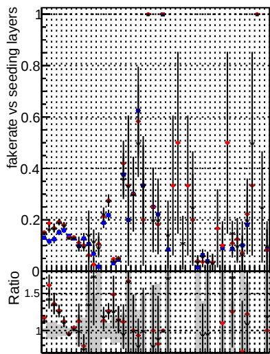
Fake rate vs. — DOM mkFit T-Original — DOM mkFit JanUpdate-noErr — DOM mkFit JanUpdate-noErr1H
