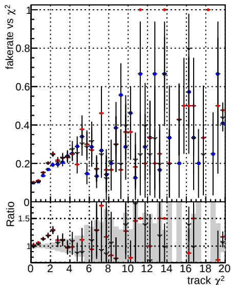
Fake rate vs. — DOM mkFit T-Original — DOM mkFit JanUpdate-noErr — DOM mkFit JanUpdate-noErr1H
