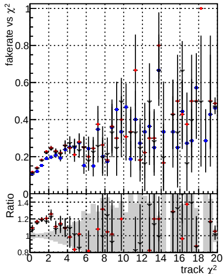
Fake rate vs. — DOM mkFit TToriginal — DOM mkFit TTJanUpdate-noErr — DOM mkFit TTJanUpdate-noErr1H
