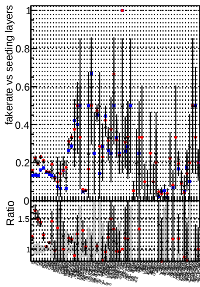
Fake rate vs. — DOM mkFit TToriginal — DOM mkFit TTJanUpdate-noErr — DOM mkFit TTJanUpdate-noErr1H
