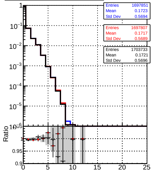
DQM_mkFit_TToriginal DQM_mkFit_TT_JanUpdate-noErr DQM_mkFit_TT_JanUpdate-noErr1H mean hits
