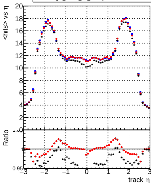
DQM_mkFit_TToriginal DQM_mkFit_TT_JanUpdate-noErr DQM_mkFit_TT_JanUpdate-noErr1H mean hits
