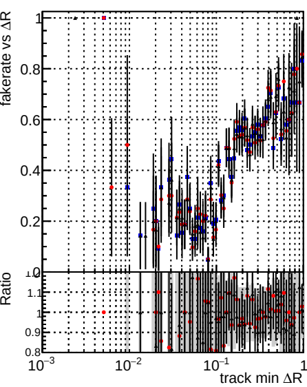
Legend: DQM_mkFit_TToriginal (blue circles), DQM_mkFit_TT_JanUpdate-noErr (red circles), DQM_mkFit_TT_JanUpdate-1H (black circles)
