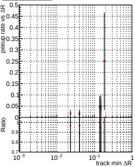
Legend: DQM_mkFit_TToriginal (blue), DQM_mkFit_TT_JanUpdate-noErr (red), DQM_mkFit_TT_JanUpdate-noErr1H (black)
