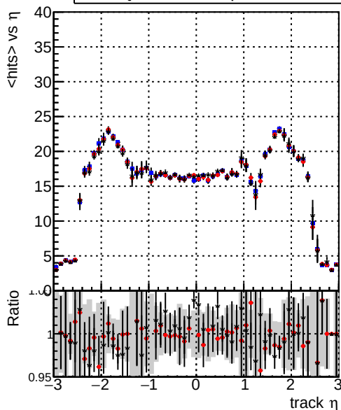
mean hit — DQM_mkFit_TToriginal — DQM_mkFit_TT_JanUpdate-noErr — DQM_mkFit_TT_JanUpdate-noErr1H
