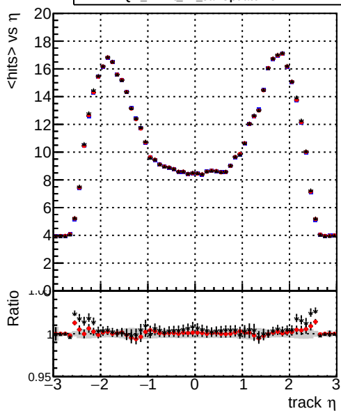
mean hits DQM_mkFit_TToriginal DQM_mkFit_TT_JanUpdate-noErr DQM_mkFit_TT_JanUpdate-noErr1H
