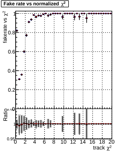
Fake rate vs. DOM mkFit TToriginal JanUpdate-noErr DOM mkFit TT JanUpdate-noErr1H
