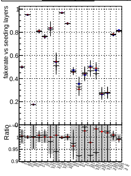
Fake rate vs. DOM mkFit TToriginal JanUpdate-noErr DOM mkFit TT JanUpdate-noErr1H
