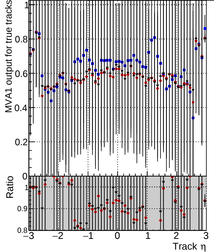
MVA1 of associated tracks (recoToSim) vs. track \eta Legend: ■ DQM_mkFit_TToriginal ● DQM_mkFit_TT_JanUpdate-noErr ▲ DQM_mkFit_TT_JanUpdate-noErr1H
