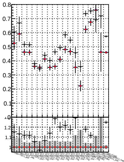
Fake rate vs. — DOM mkFit time — DOM mkFit time + b1 — DOM BDT mkFit time
