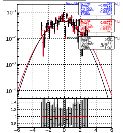
RecoAllAssoc2GenMatchedMerged_PulIZ
