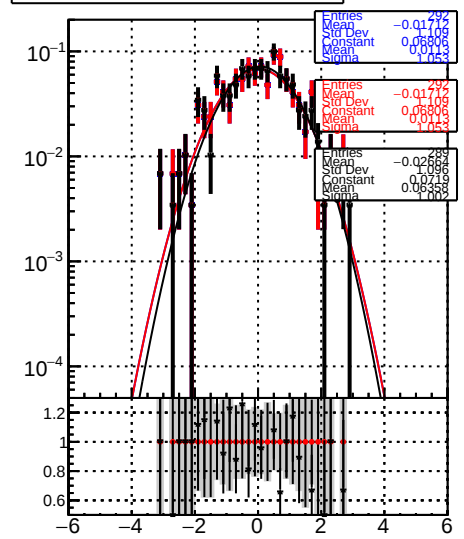
RecoAllAssoc2GenMatchedMerged_PulIX
