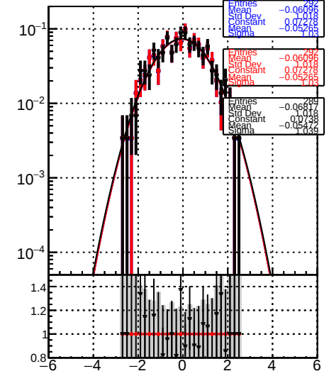
RecoAllAssoc2GenMatchedMerged_PulIZ
