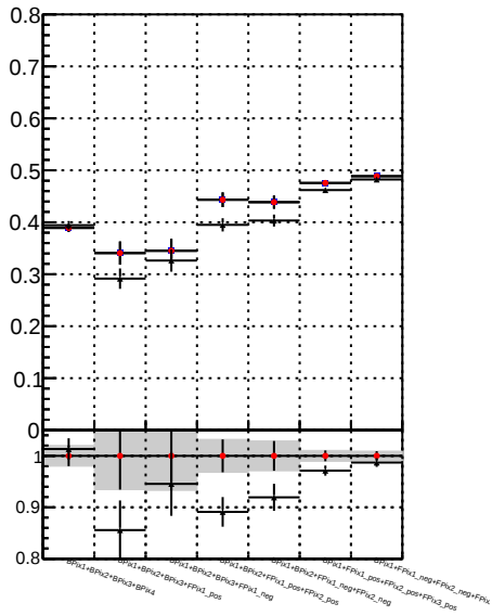
Fake rate vs. DOM mkFit time DOM BDT mkFit time DOM BDT mkFit time
