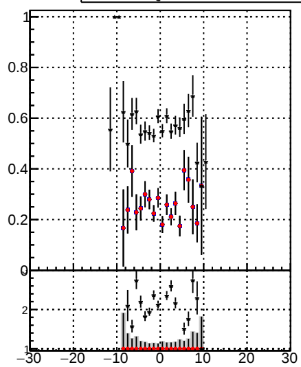
Fake rate vs v Legend: DQM_mkFit_time (black line with dots) DQM_mkFit_time_b1 (red line with dots) DQM_BDT_mkFit_time (black line with dots)
