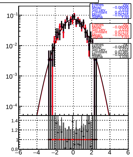
RecoAllAssoc2GenMatchedMerged_PulIZ
