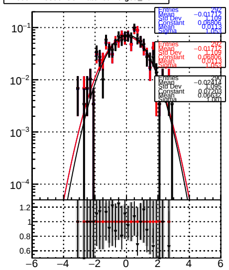
RecoAllAssoc2GenMatchedMerged_PulIX
