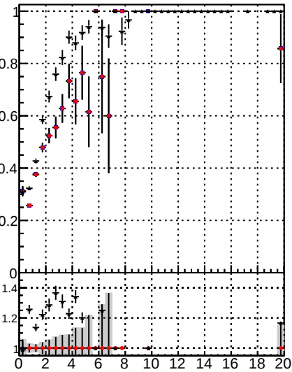
Fake rate vs. — DOM mkFit time — DOM BDT mkFit time — DOM BDT mkFit time b1
