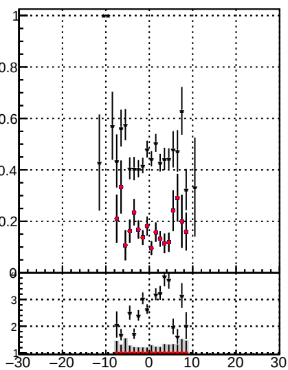
Fake rate vs d Legend: DOM mkFit time DOM mkFit time b1 DOM BDT mkFit time
