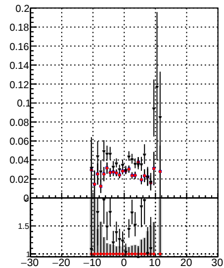
Fake rate vs d —•— DOM mkFit time —•— DOM mkFit time b1 —•— DOM BDT mkFit time
